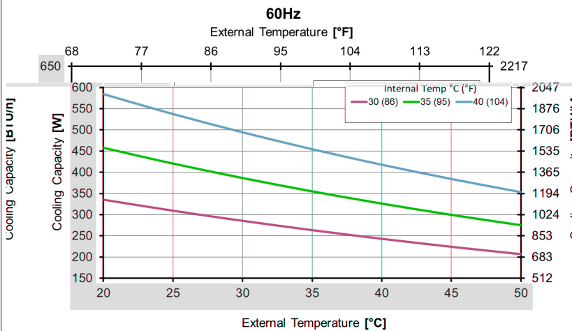
Cooling Capacity vs Temperature
